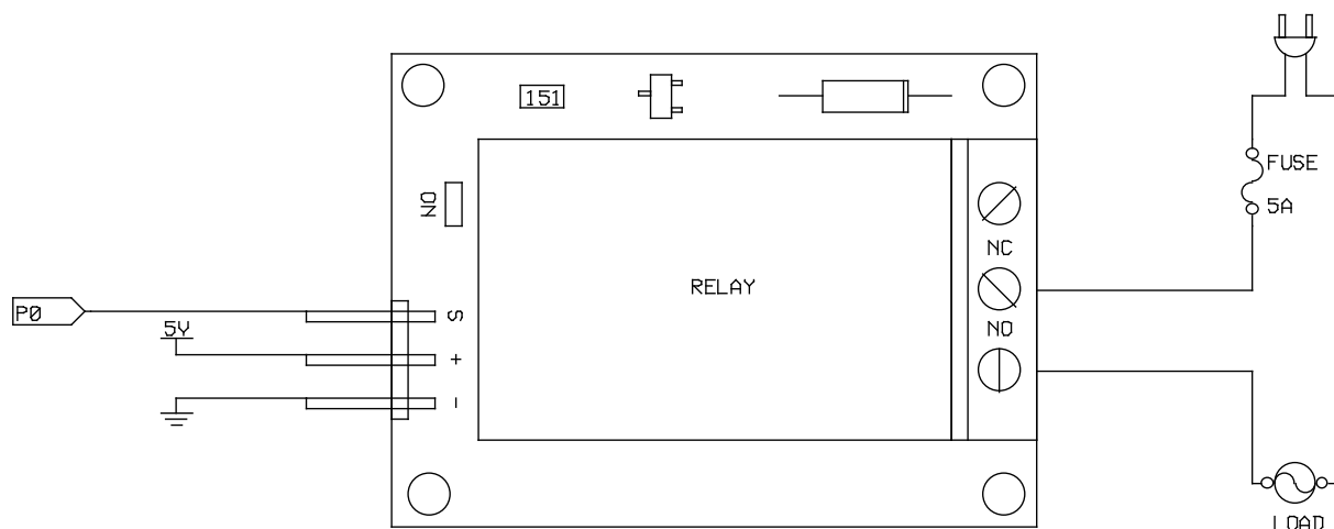
Figure 1: Connection Example
