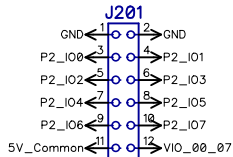
2x6 Pin Header
