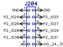
2x6 Pin Header
