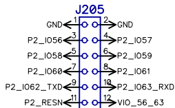
2x6 Pin Header
