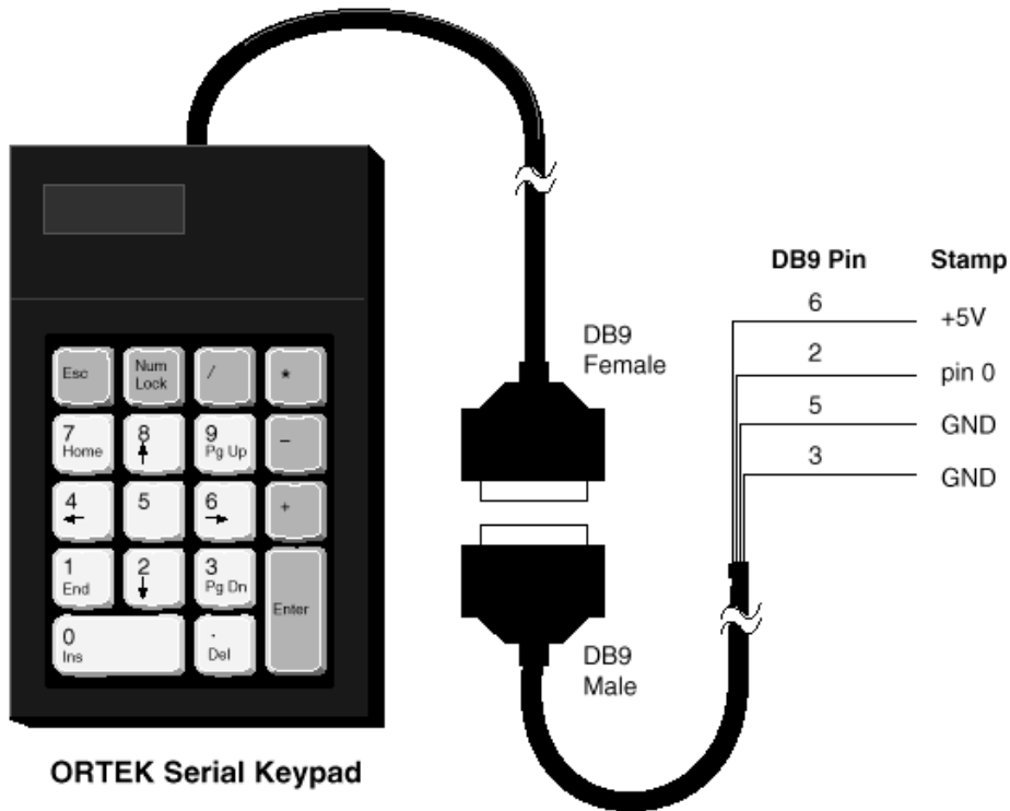
Figure 3.1: Connecting the serial keypad to the Stamp for data entry requires just one I/O pin plus a few microamps from the Stamp's power supply.
