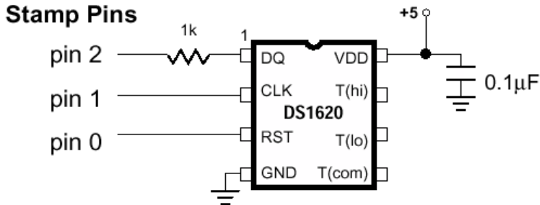
Figure 2.2: DS1620 Pinout and Connection
