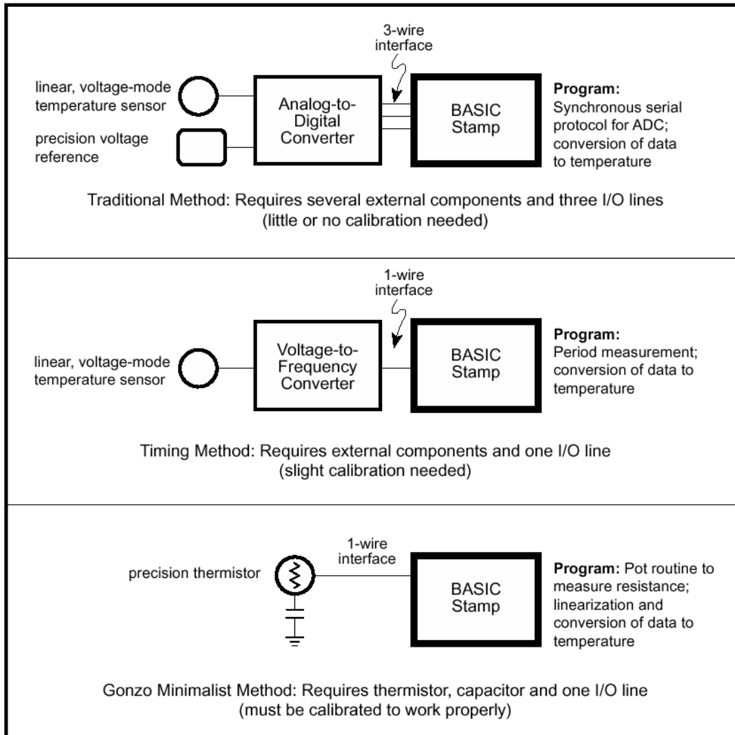
Figure 2.1: Three methods for measuring temperature with the Stamp
